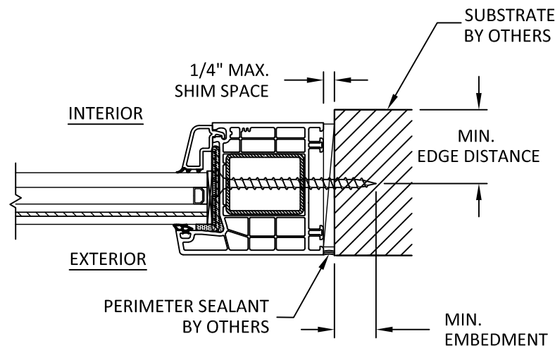
A 6 ANCHOR DETAIL THROUGH FRAME (JAMB)
