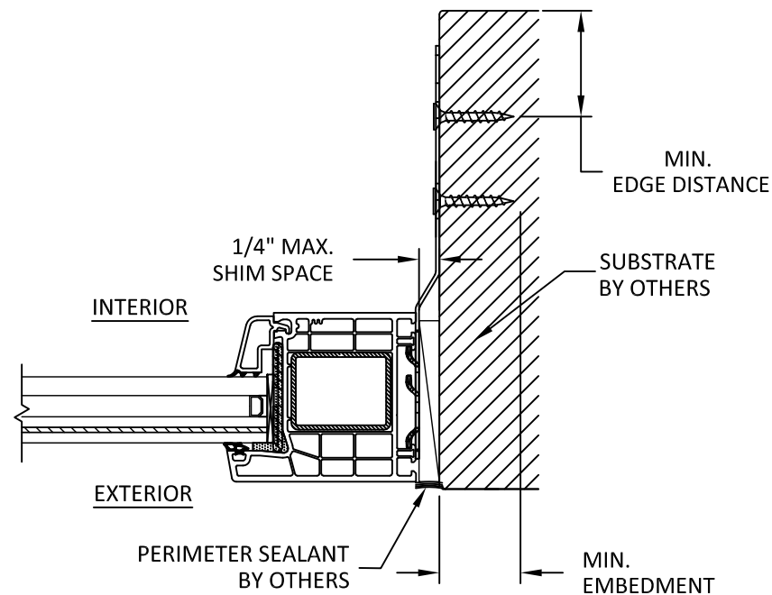
B 6 ANCHOR DETAIL STRAP (JAMB)
