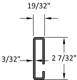
8 REINFORCEMENT
